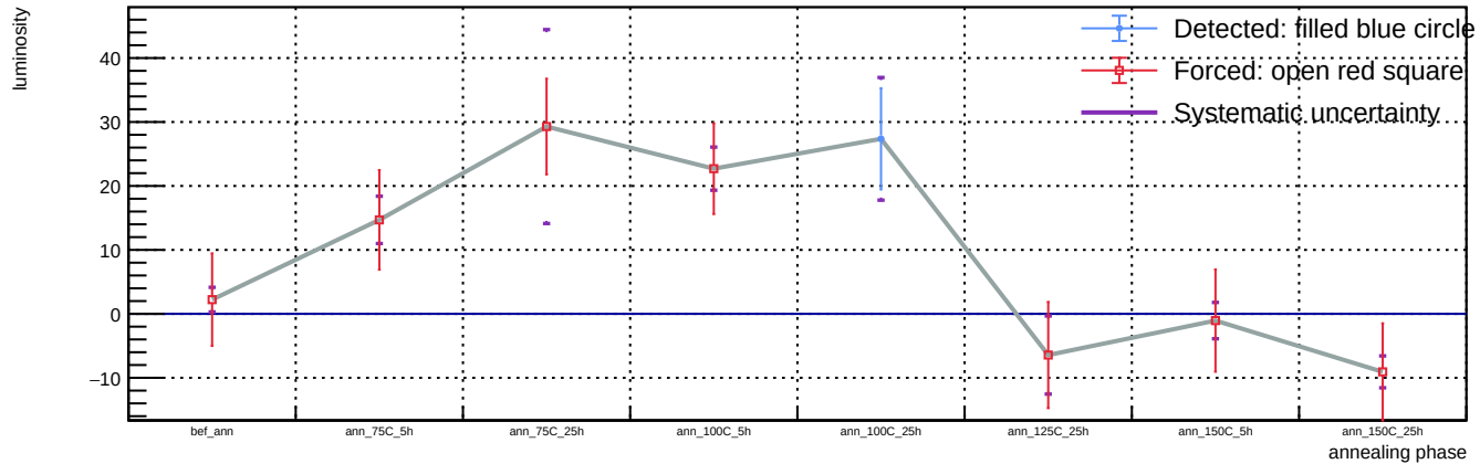
Sensor A1, v = 5 V, representative T = 23 C (max available) - Spot 76: luminosity vs phase
