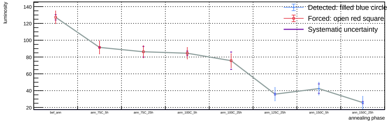
Sensor A1, v = 5 V, representative T = 23 C (max available) - Spot 86: luminosity vs phase
