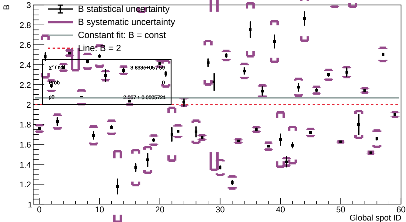
Sensor A1 - Power-law exponent B - before annealing
