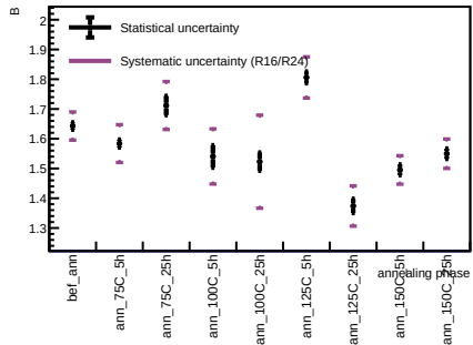
Sensor A1, T = 20 C - Spot 19
