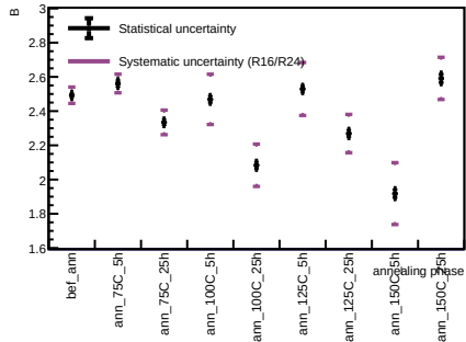
Sensor A1, T = 20 C - Spot 31
