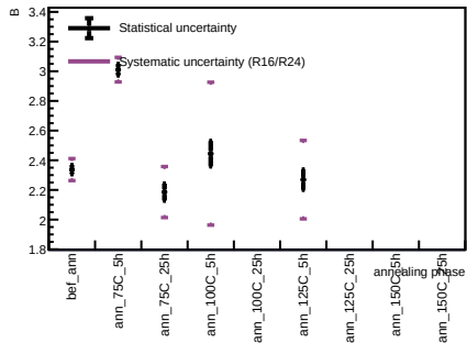
Sensor A1, T = 20 C - Spot 34
