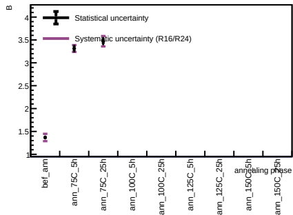
Sensor A1, T = 20 C - Spot 30
