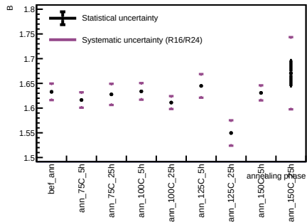
Sensor A1, T = 20 C - Spot 33
