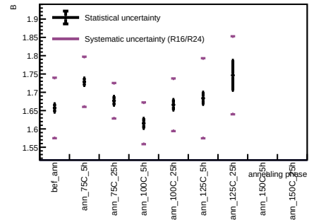
Sensor A1, T = 20 C - Spot 56
