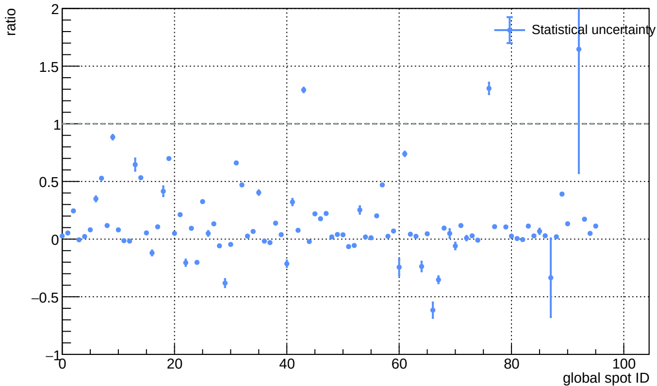
Sensor A1, T = 20 C - L(\text{ann\_150C\_25h}) / L(\text{before\_annealing})
