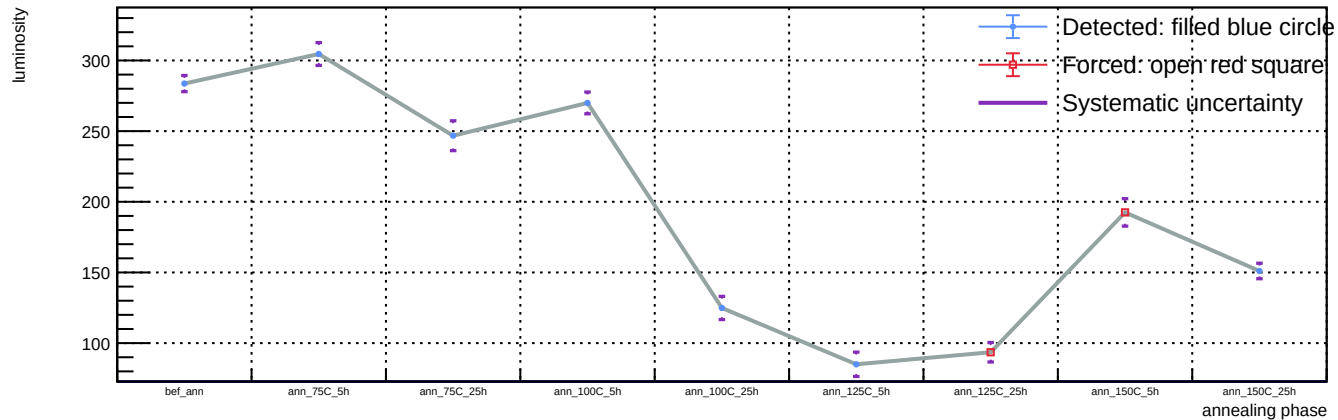
Sensor A1, T = 20 C, representative v = 58.3 V (max available) - Spot 14: luminosity vs phase
