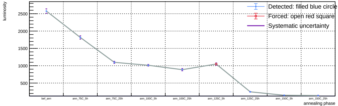
Sensor A1, T = 20 C, representative v = 58.3 V (max available) - Spot 15: luminosity vs phase
