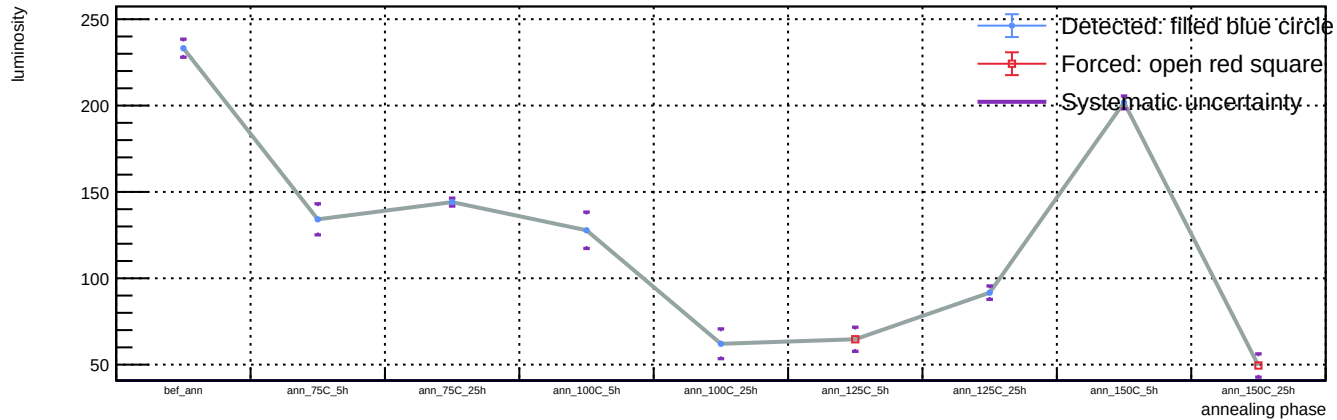
Sensor A1, T = 20 C, representative v = 58.3 V (max available) - Spot 21: luminosity vs phase
