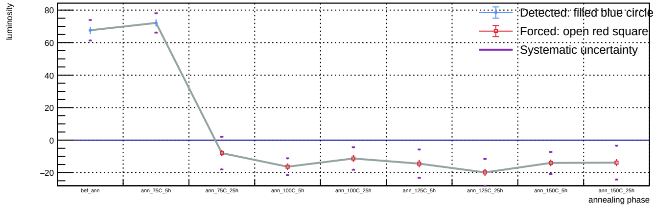
Sensor A1, T = 20 C, representative v = 58.3 V (max available) - Spot 22: luminosity vs phase
