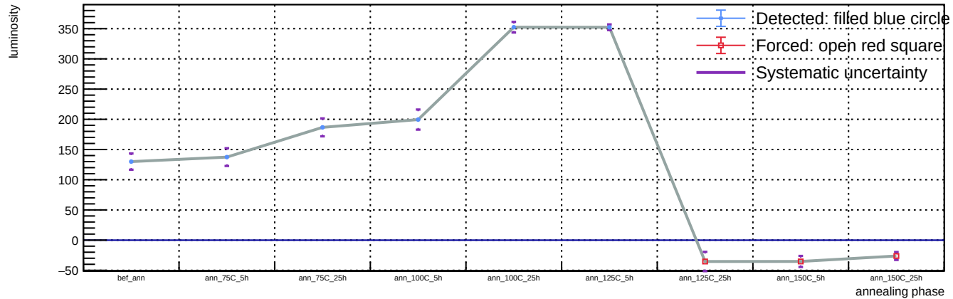
Sensor A1, T = 20 C, representative v = 58.3 V (max available) - Spot 24: luminosity vs phase
