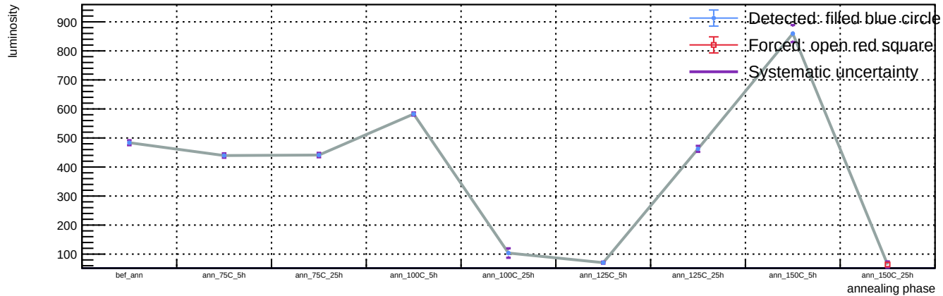
Sensor A1, T = 20 C, representative v = 58.3 V (max available) - Spot 27: luminosity vs phase
