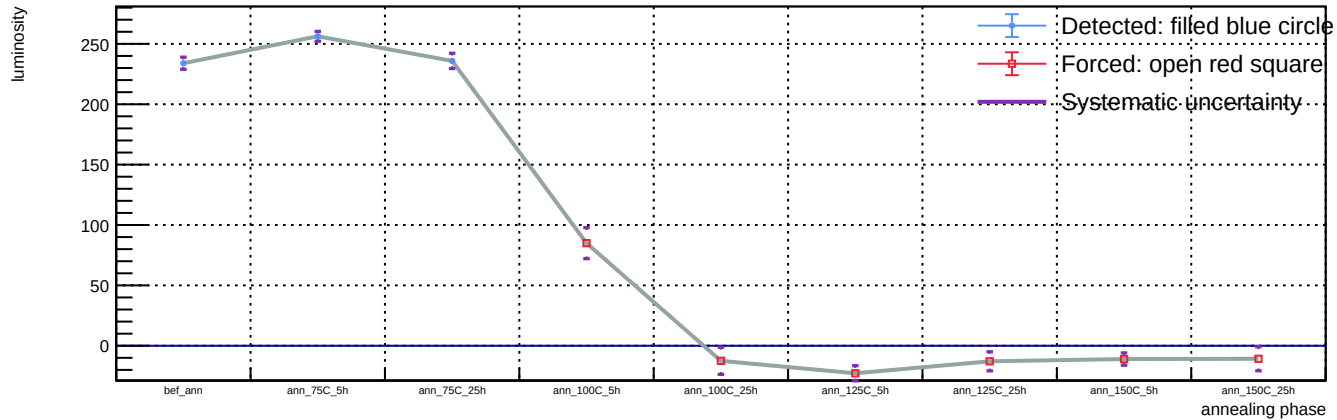
Sensor A1, T = 20 C, representative v = 58.3 V (max available) - Spot 30: luminosity vs phase
