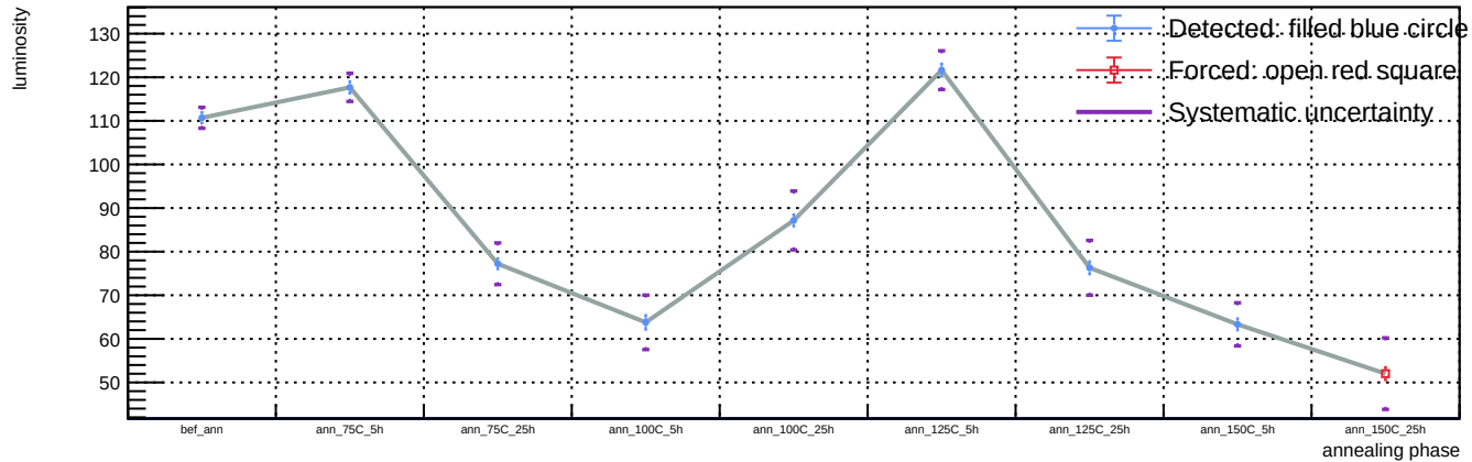
Sensor A1, T = 20 C, representative v = 58.3 V (max available) - Spot 32: luminosity vs phase
