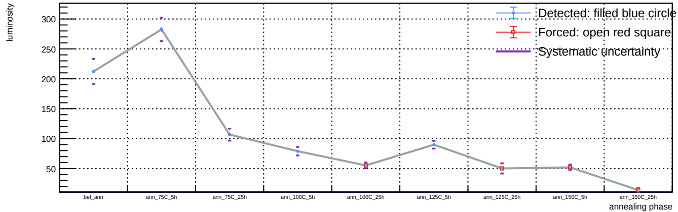
Sensor A1, T = 20 C, representative v = 58.3 V (max available) - Spot 34: luminosity vs phase
