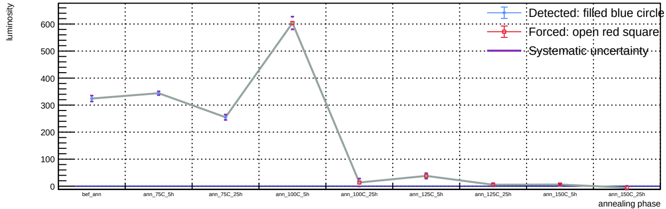
Sensor A1, T = 20 C, representative v = 58.3 V (max available) - Spot 36: luminosity vs phase
