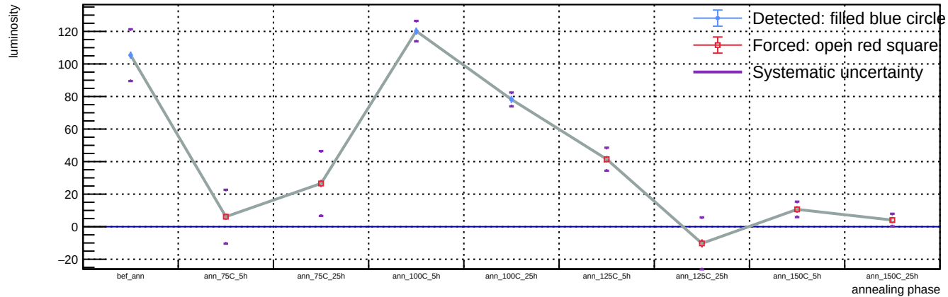
Sensor A1, T = 20 C, representative v = 58.3 V (max available) - Spot 39: luminosity vs phase
