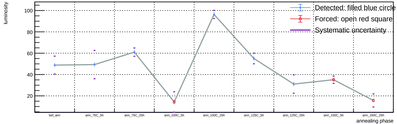
Sensor A1, T = 20 C, representative v = 58.3 V (max available) - Spot 41: luminosity vs phase
