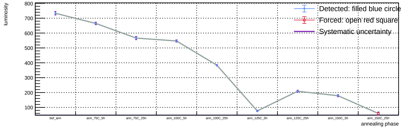
Sensor A1, T = 20 C, representative v = 58.3 V (max available) - Spot 5: luminosity vs phase
