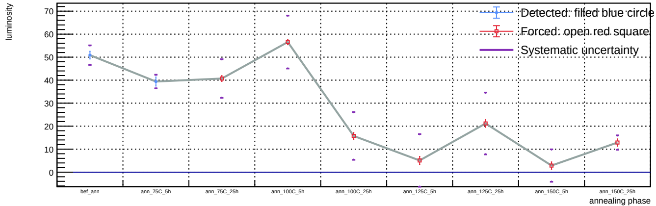
Sensor A1, T = 20 C, representative v = 58.3 V (max available) - Spot 53: luminosity vs phase
