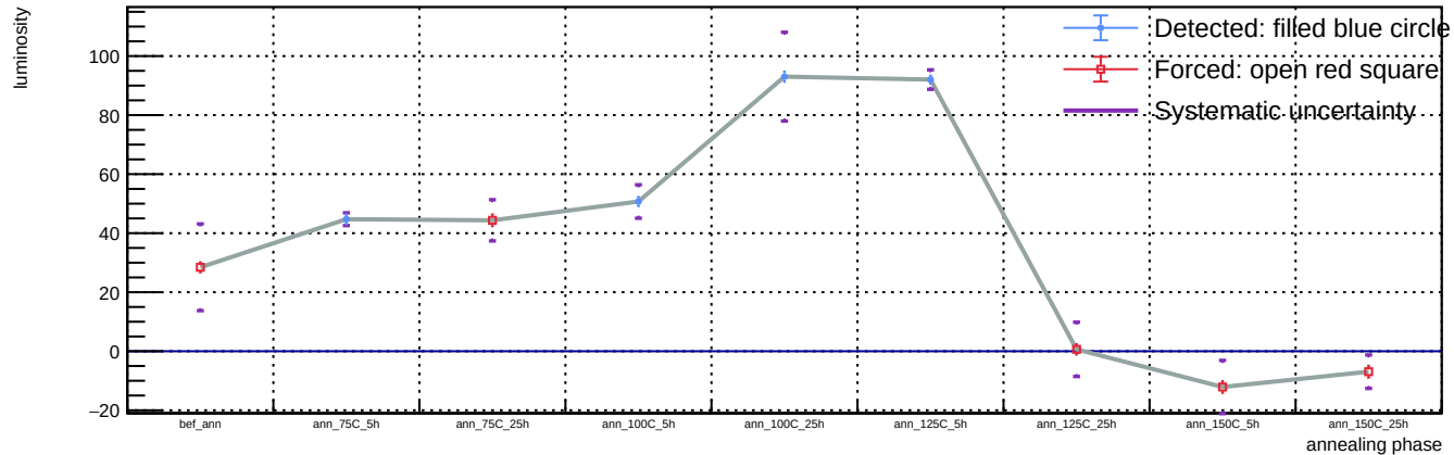
Sensor A1, T = 20 C, representative v = 58.3 V (max available) - Spot 60: luminosity vs phase
