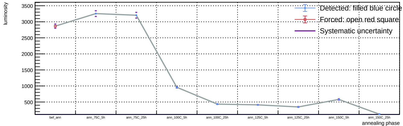
Sensor A1, T = 20 C, representative v = 58.3 V (max available) - Spot 62: luminosity vs phase
