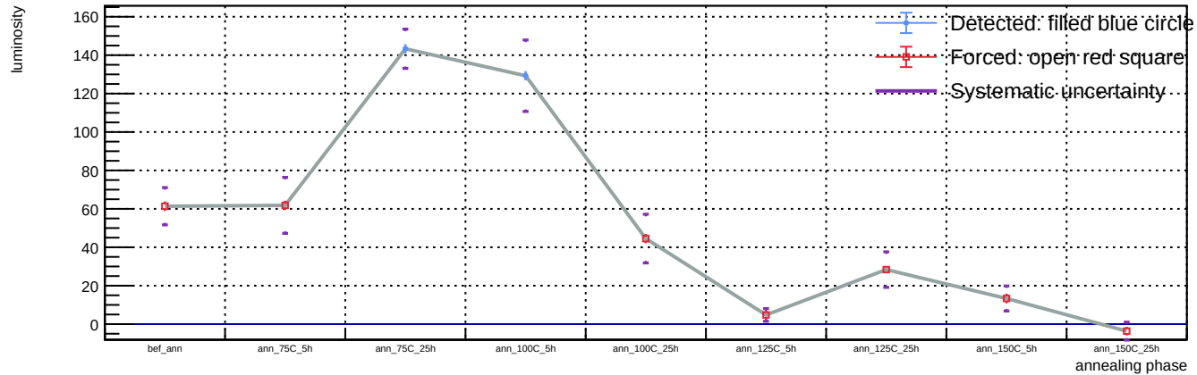
Sensor A1, T = 20 C, representative v = 58.3 V (max available) - Spot 70: luminosity vs phase
