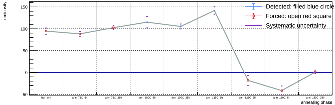
Sensor A1, T = 20 C, representative v = 58.3 V (max available) - Spot 72: luminosity vs phase
