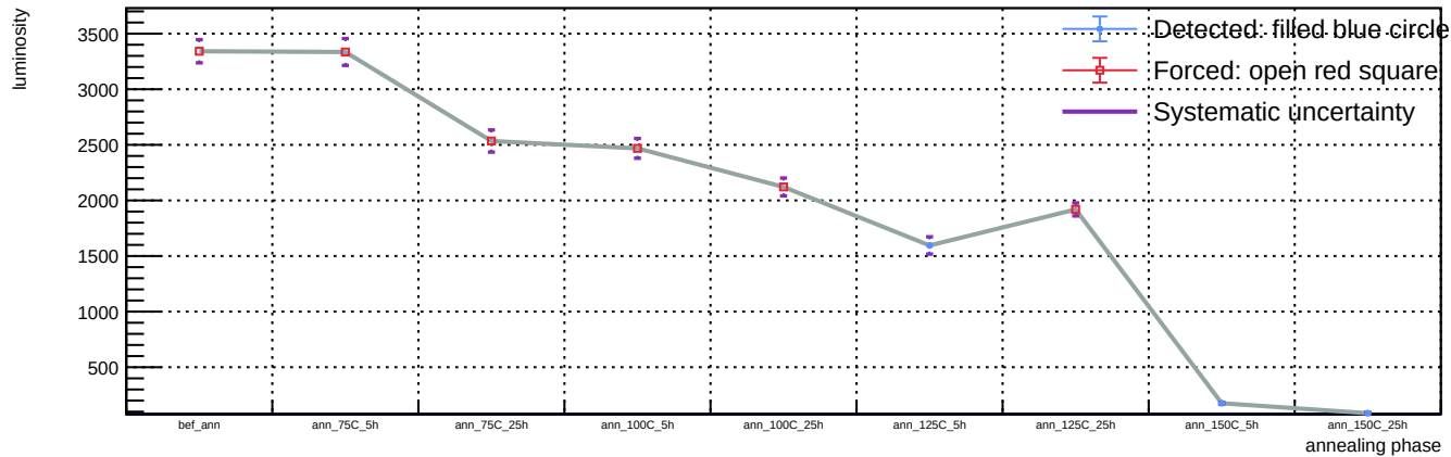
Sensor A1, T = 20 C, representative v = 58.3 V (max available) - Spot 80: luminosity vs phase
