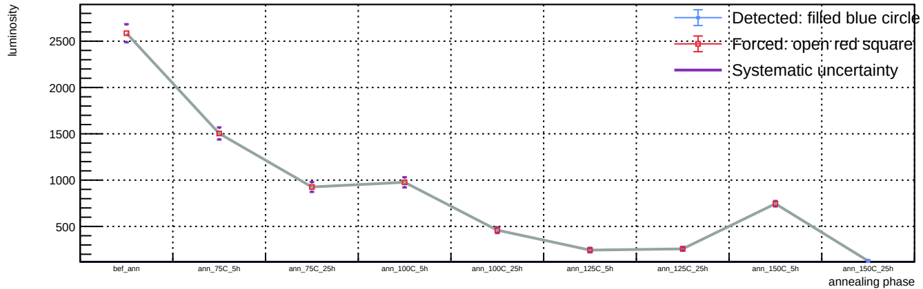
Sensor A1, T = 20 C, representative v = 58.3 V (max available) - Spot 94: luminosity vs phase
