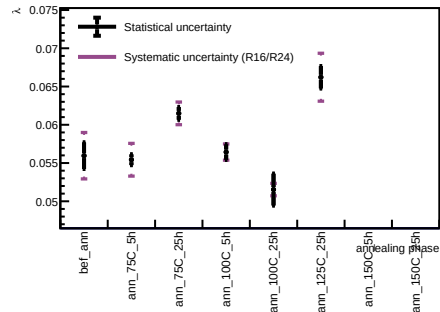
Sensor A1, v = 5 V - Spot 8
