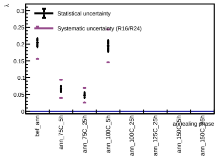
Sensor A1, v = 5 V - Spot 18
