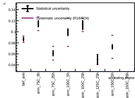
Sensor A1, v = 5 V - Spot 21
