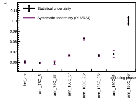
Sensor A1, v = 5 V - Spot 20
