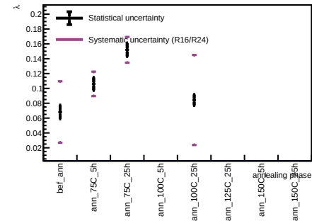
Sensor A1, v = 5 V - Spot 41
