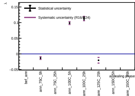
Sensor A1, v = 5 V - Spot 68
