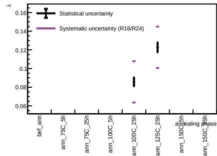
Sensor A1, v = 5 V - Spot 74
