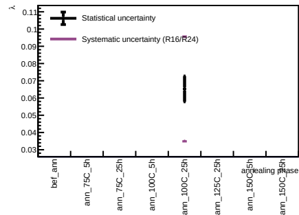
Sensor A1, v = 5 V - Spot 77
