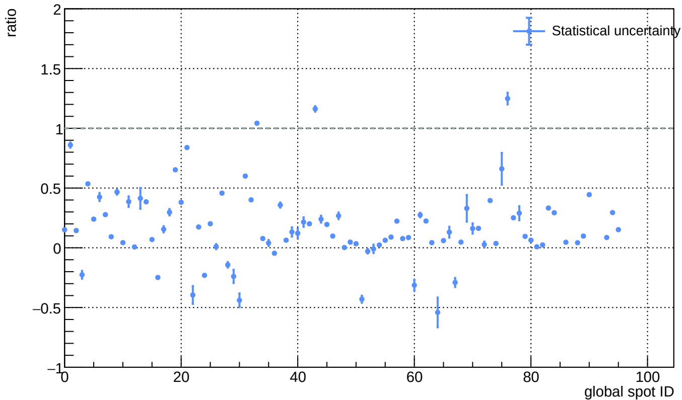
Sensor A1, v = 5 V - L(\text{ann\_150C\_5h}) / L(\text{before\_annealing})
