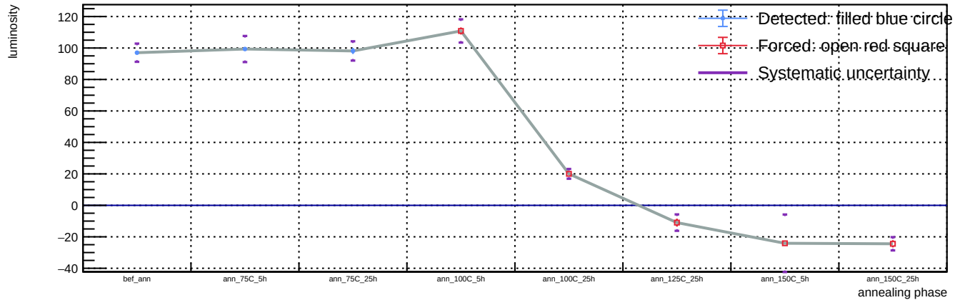
Sensor A1, v = 5 V, representative T = 23 C (max available) - Spot 16: luminosity vs phase
