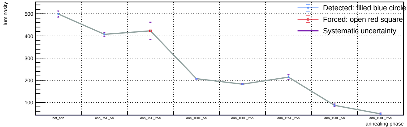
Sensor A1, v = 5 V, representative T = 23 C (max available) - Spot 23: luminosity vs phase
