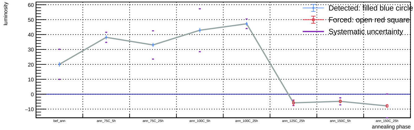
Sensor A1, v = 5 V, representative T = 23 C (max available) - Spot 29: luminosity vs phase
