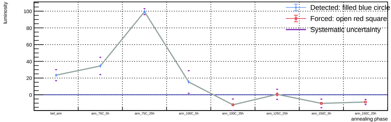
Sensor A1, v = 5 V, representative T = 23 C (max available) - Spot 30: luminosity vs phase
