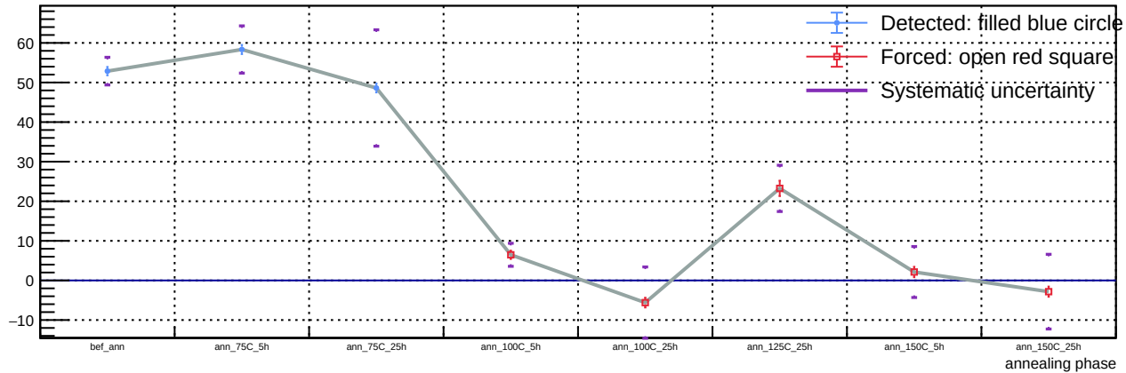
Sensor A1, v = 5 V, representative T = 23 C (max available) - Spot 35: luminosity vs phase
