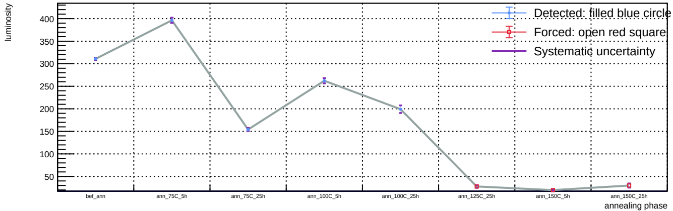
Sensor A1, v = 5 V, representative T = 23 C (max available) - Spot 38: luminosity vs phase
