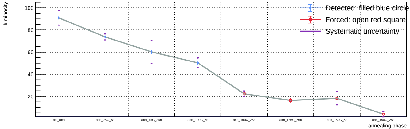
Sensor A1, v = 5 V, representative T = 23 C (max available) - Spot 42: luminosity vs phase
