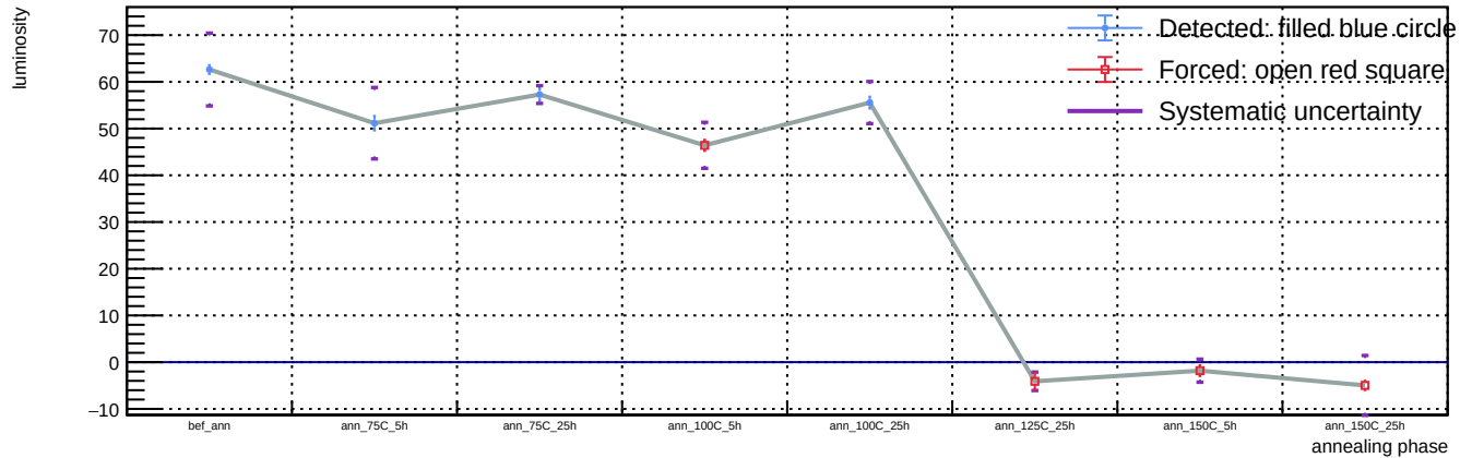
Sensor A1, v = 5 V, representative T = 23 C (max available) - Spot 52: luminosity vs phase
