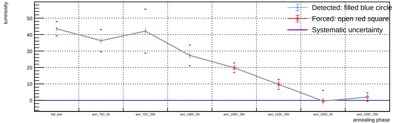
Sensor A1, v = 5 V, representative T = 23 C (max available) - Spot 53: luminosity vs phase
