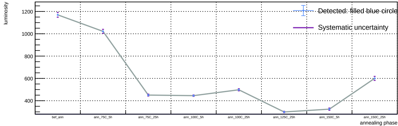
Sensor A1, v = 5 V, representative T = 23 C (max available) - Spot 7: luminosity vs phase
