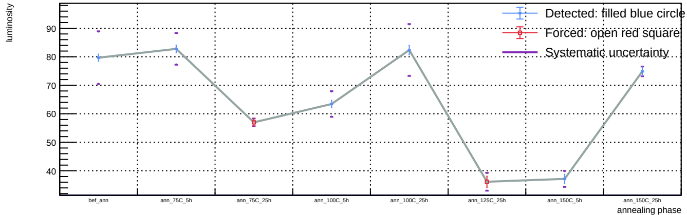
Sensor A1, v = 5 V, representative T = 23 C (max available) - Spot 9: luminosity vs phase
