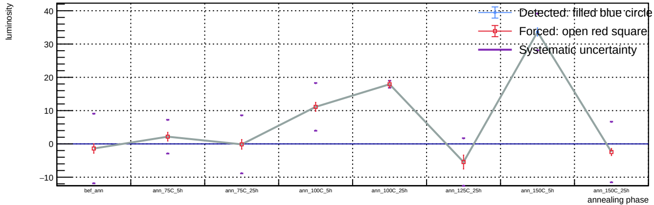
Sensor A1, v = 5 V, representative T = 23 C (max available) - Spot 92: luminosity vs phase
