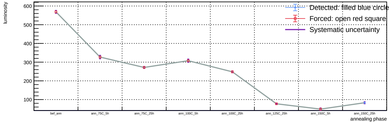
Sensor A1, v = 5 V, representative T = 23 C (max available) - Spot 93: luminosity vs phase
