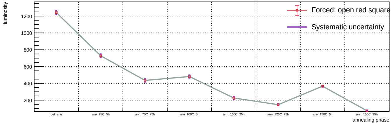
Sensor A1, v = 5 V, representative T = 23 C (max available) - Spot 94: luminosity vs phase
