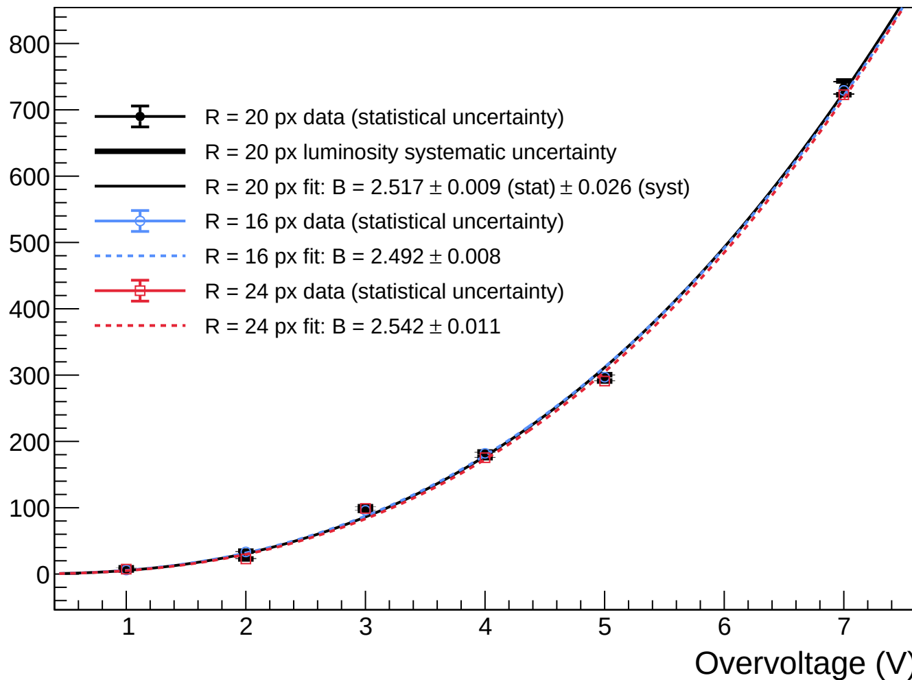
Spot 5: x = 193.70, y = 520.10, T = 20.0 °C before_annealing
