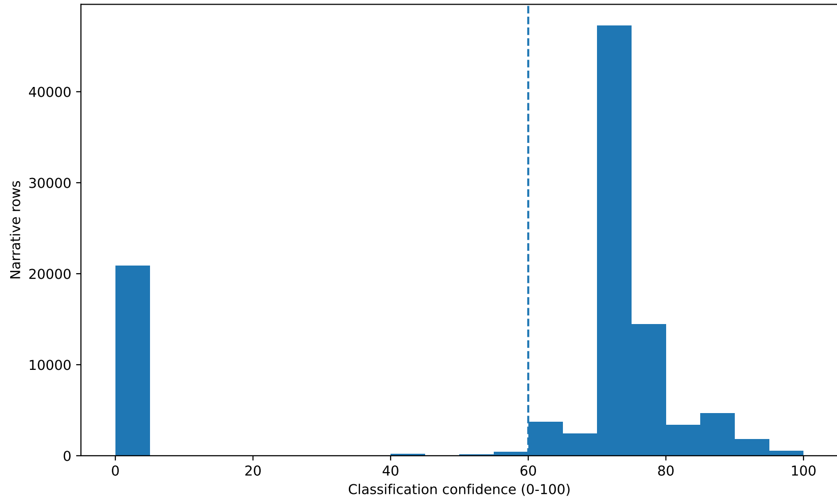
openai-gpt-5-nano row-level classification confidence
