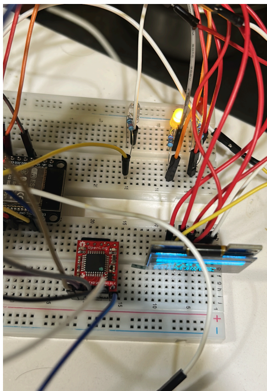
Figure 3: SparkFun Logger connected to Breadboard
